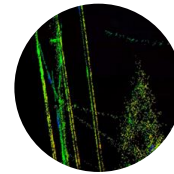
BORESIGHT CALIBRATION
