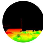
GEOREFERENCING
