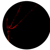
TRAJECTORY PROCESSING
