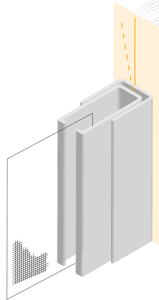
Telescopic system
