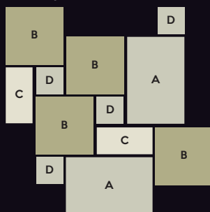
A 871x580 mm C 580x288 mm B 580x580 mm D 288x288 mm
