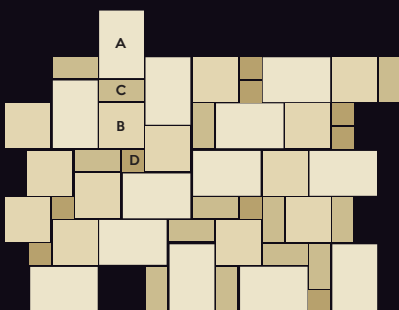
A 900x600 mm - 13 pcs C 600x290 mm - 13 pcs B 600x600 mm - 13 pcs D 290x290 mm - 9 pcs
